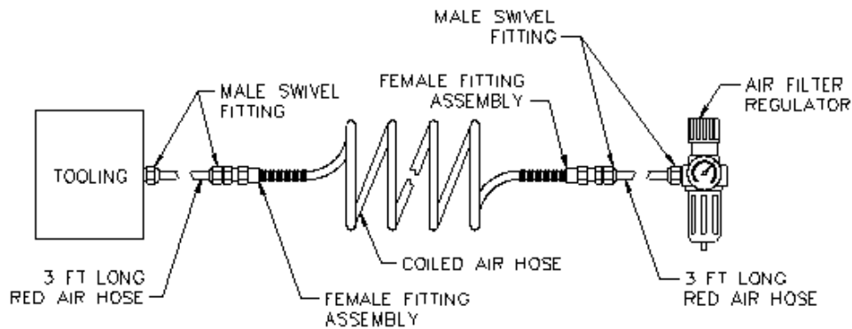
Diagram 2. Air hose assembly.
