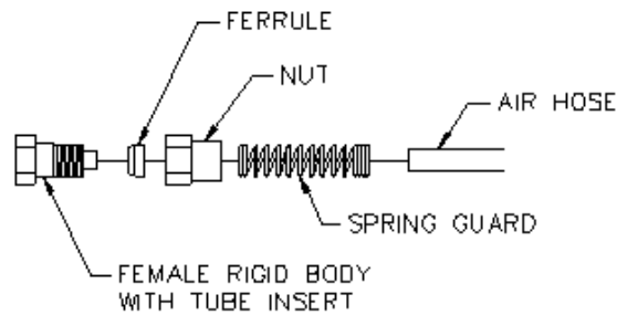
Diagram 1. Female fitting assembly
